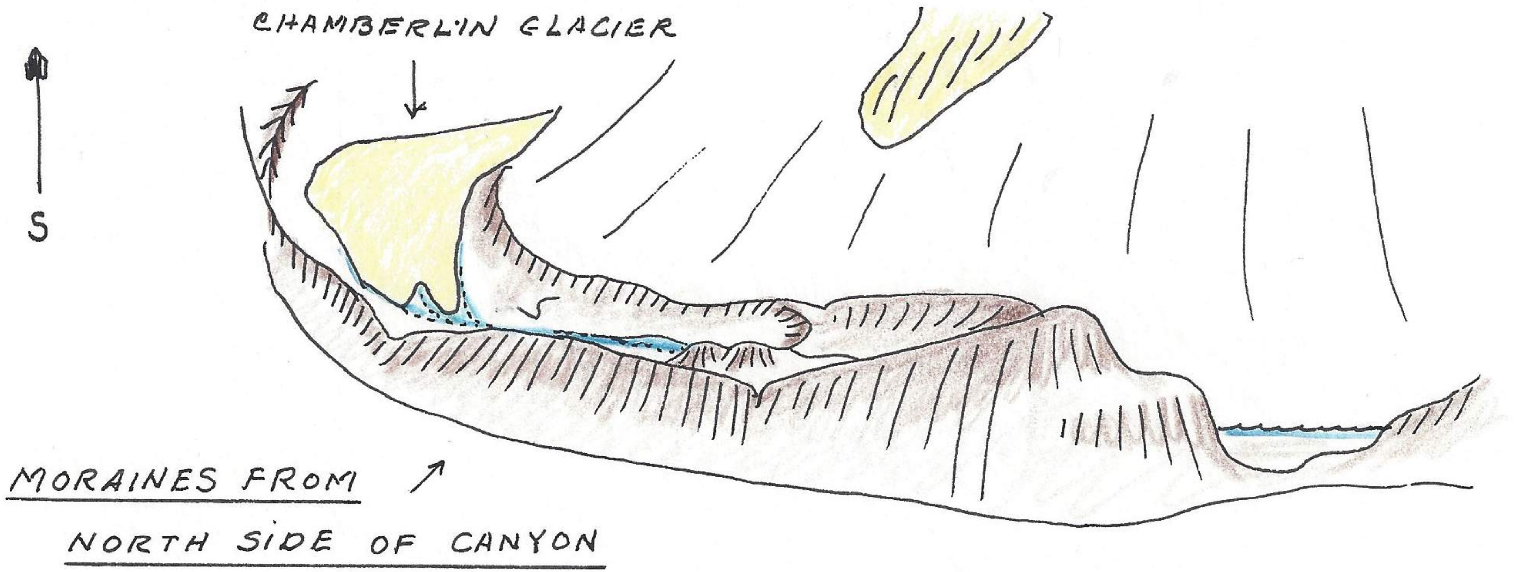
GLACIER ON MT. SLOPE
