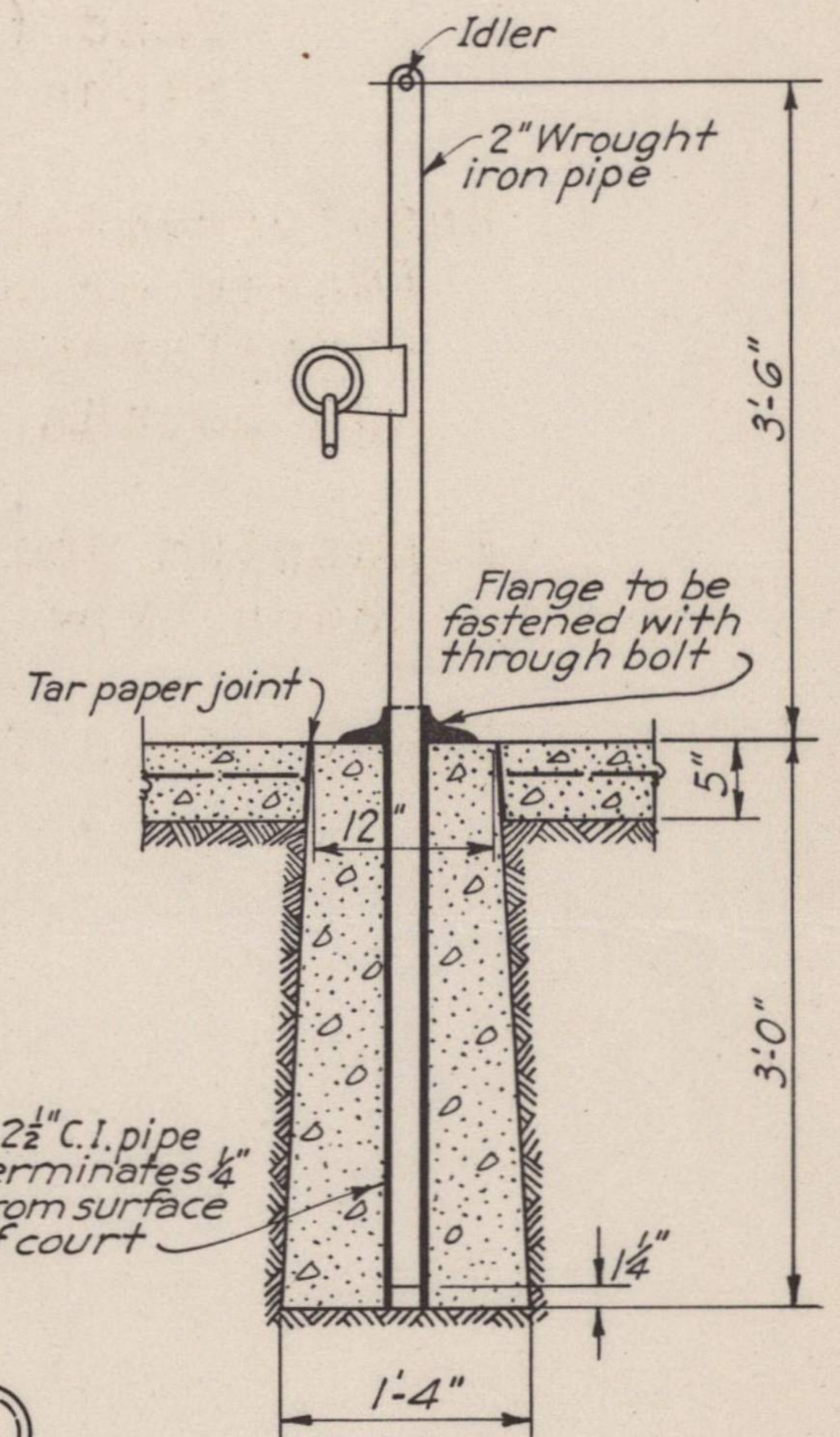
REMOVABLE PIPE POST
