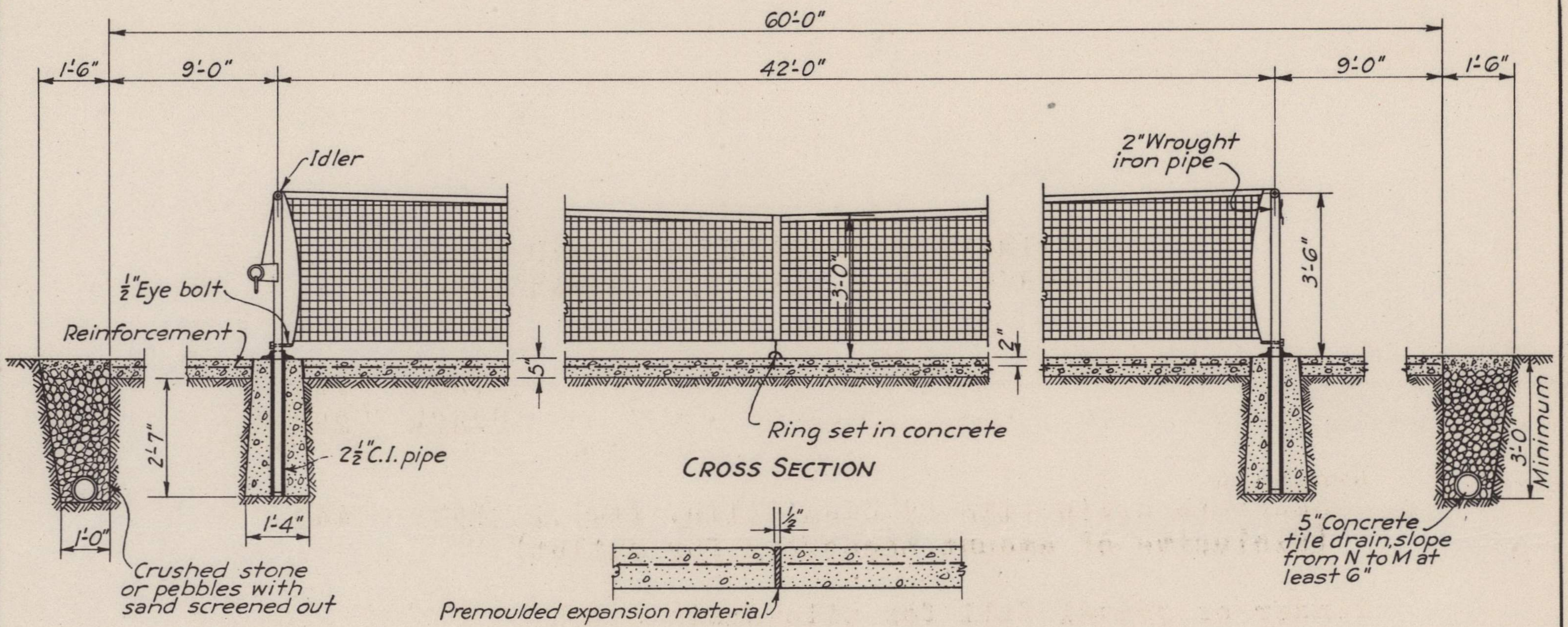
DETAIL OF EXPANSION JOINT
