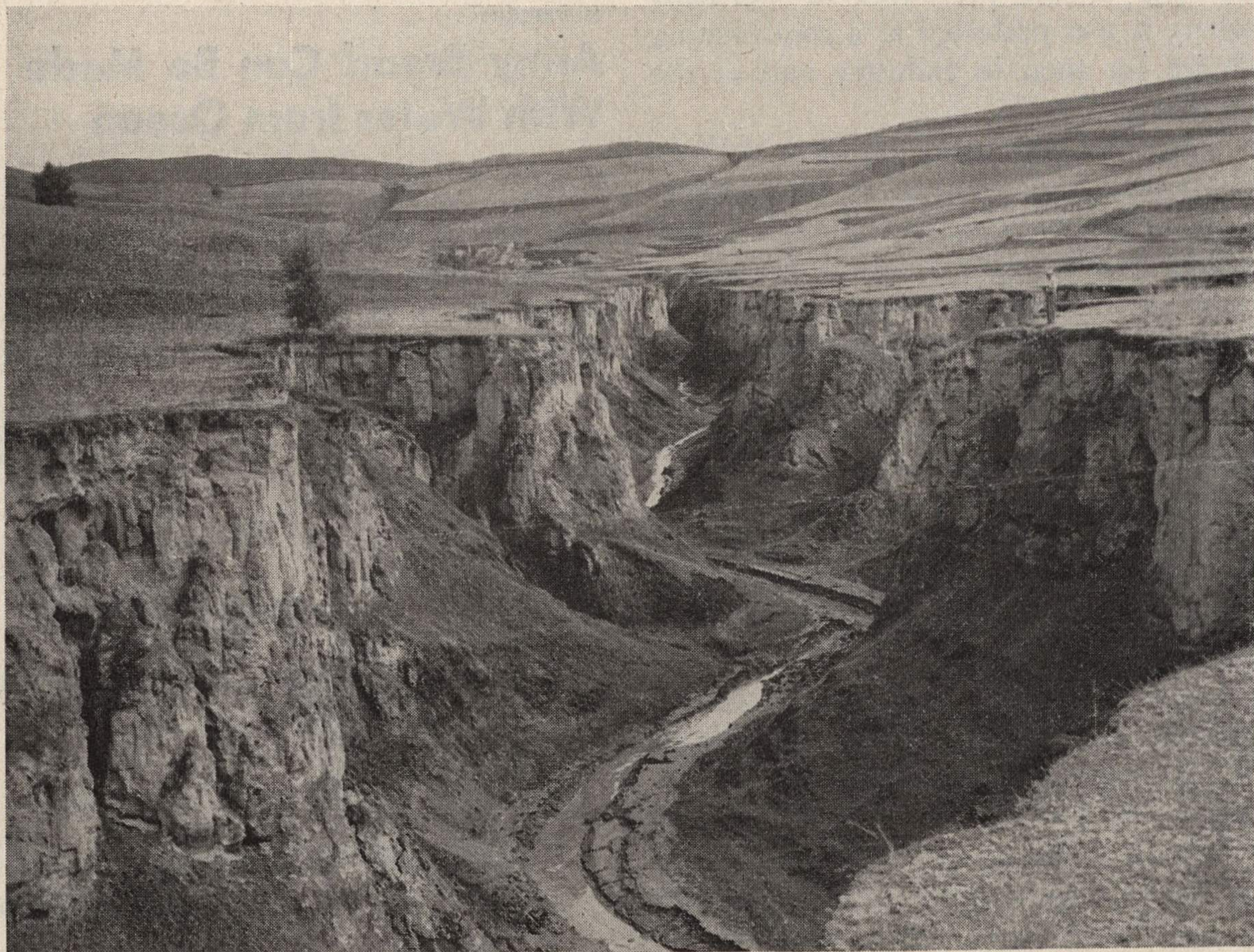
CUT BY EROSION —Accelerated wearing away leaves deep gullies such as this one which dwarfs the man at the right. Some of these gullies are as much as 800 feet deep. This photograph, taken in Kansu, China, was made by Dr. W. C. Lowdermilk, as were the beautiful pictures of China shown on these pages and of the yak on the cover of this SCIENCE NEWS LETTER .
