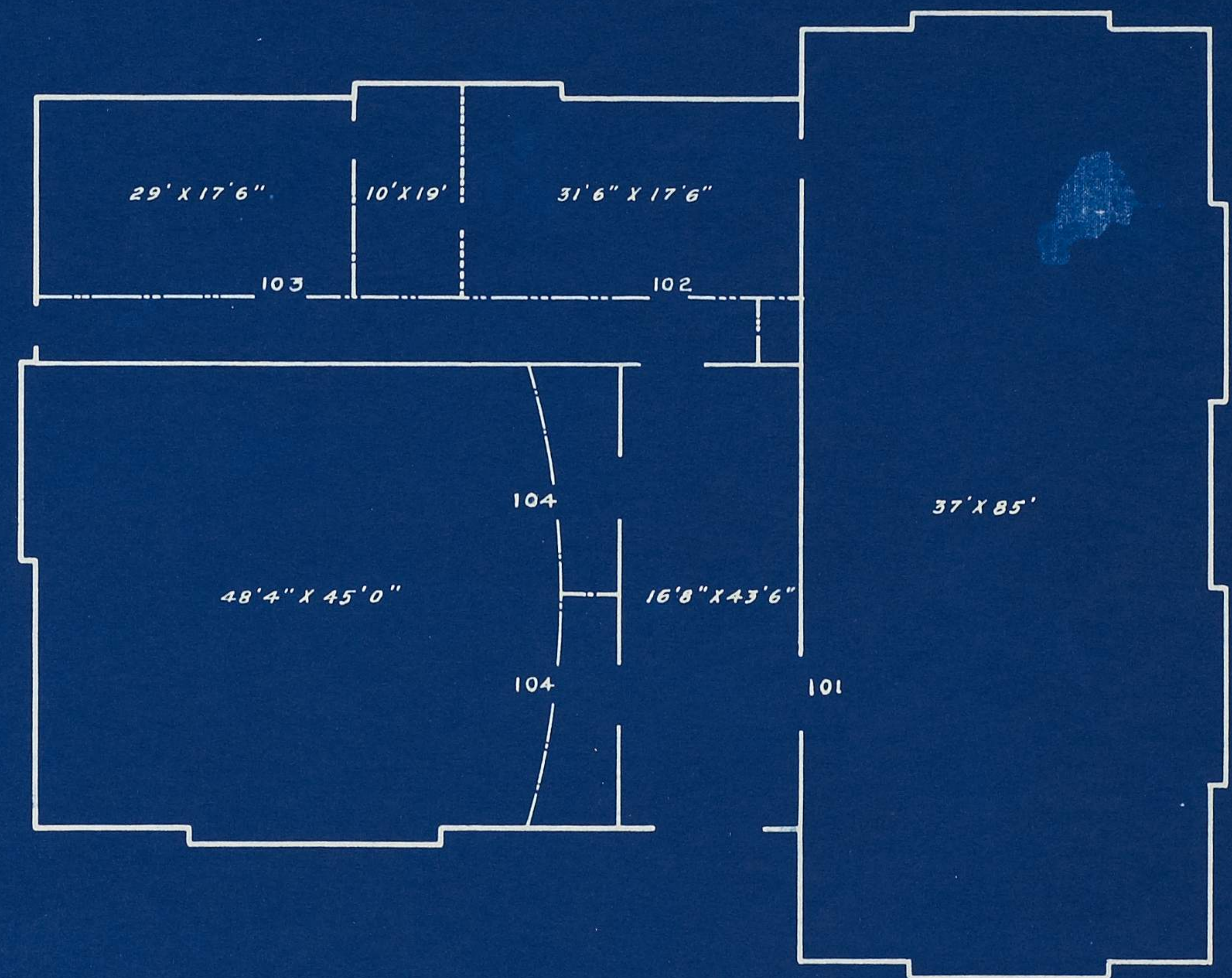
PLAN OF FIRST FLOOR
