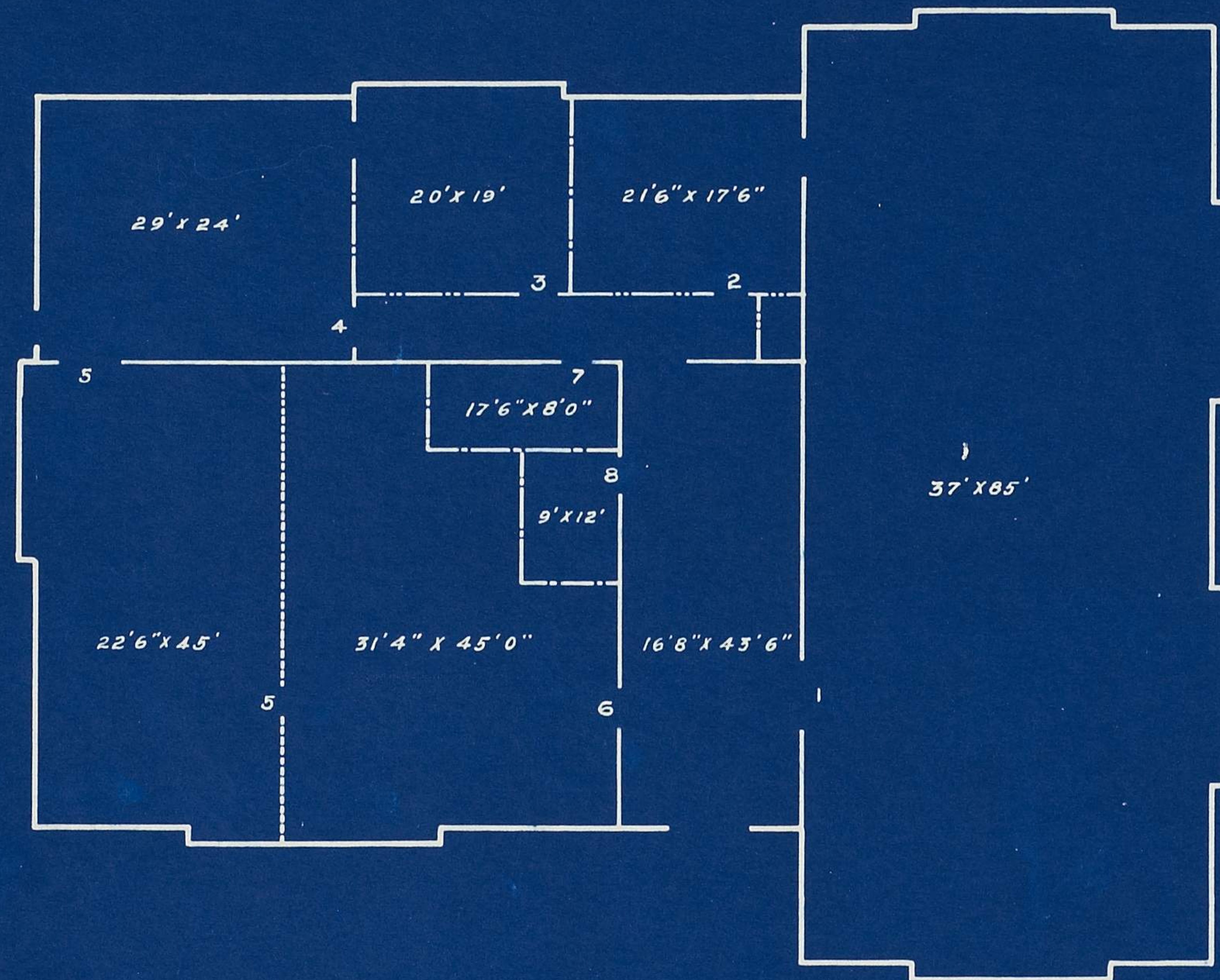
PLAN OF BASEMENT
