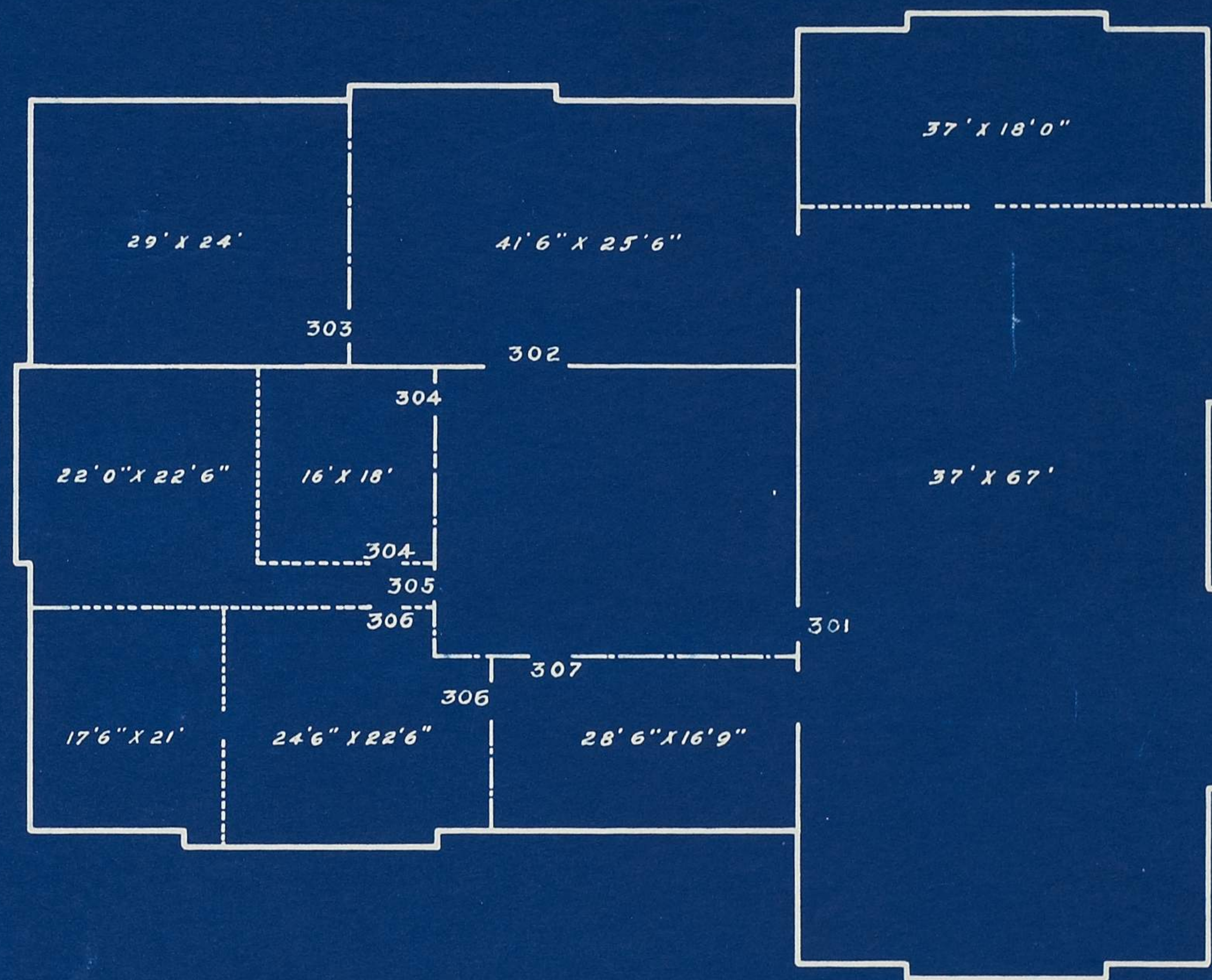
PLAN OF ATTIC FLOOR
